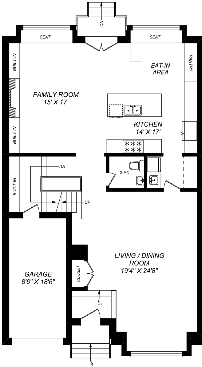
MAIN FLOOR 1314 SQUARE FEET (CEILING HEIGHT : 9'-0")
