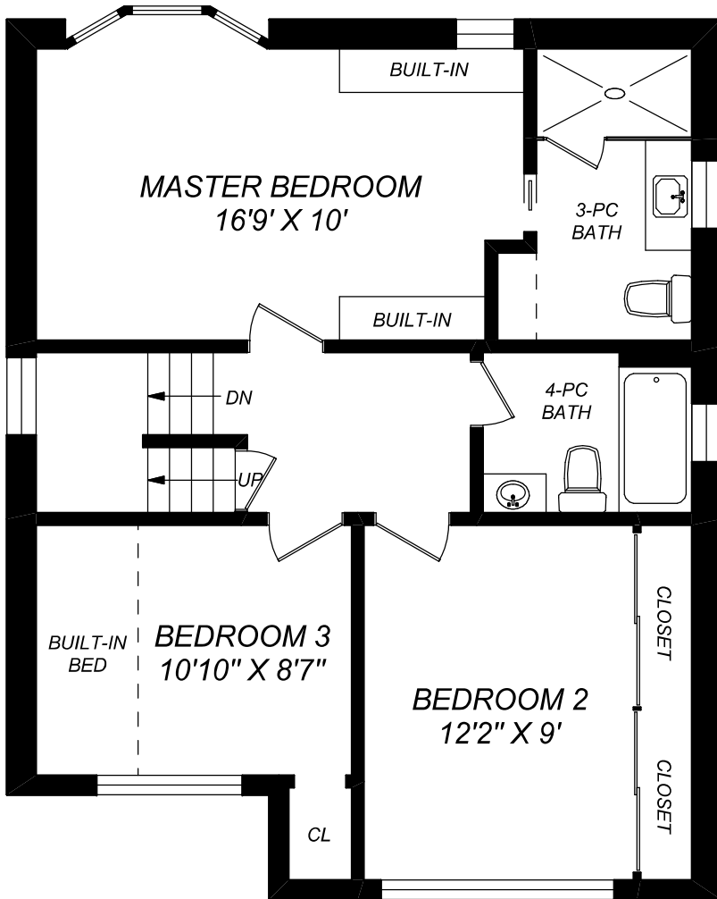
SECOND FLOOR 727 SQUARE FEET
